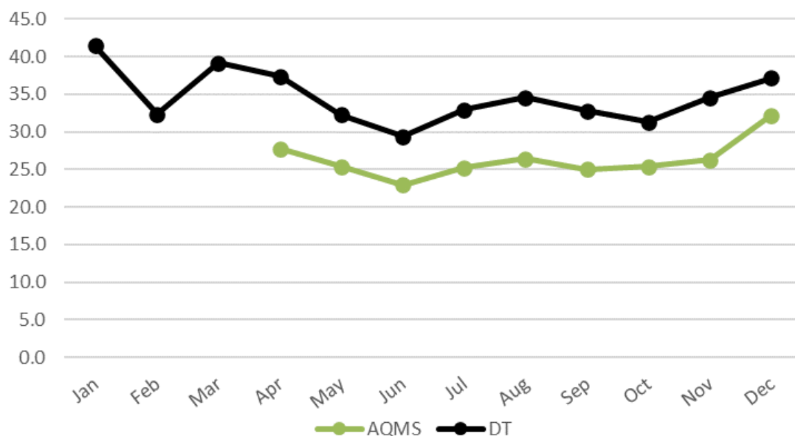
Figure 1: Comparison of Diffusion Tube and Automatic Monitoring Station Measurements at Co-located Site
